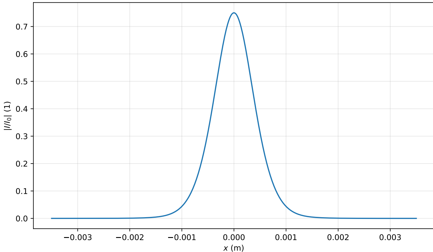
Intensity profile I(x, y = 0, z = 2.707m)/I_0 , P_{in}=0.6P_{cr} , artificial time
